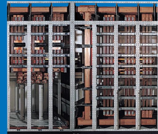
7000A Bus Bar System with Main Breaker IEC application
